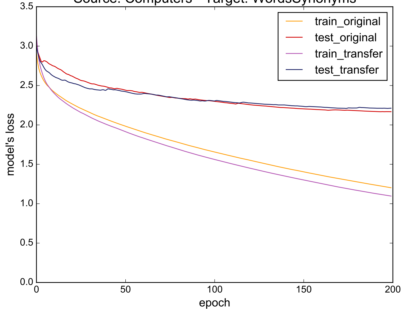
Source: Computers - Target: WordsSynonyms
