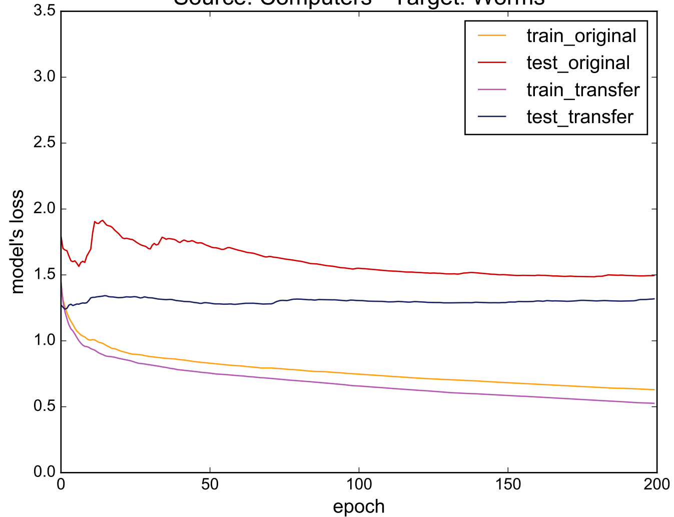
Source: Computers - Target: Worms
