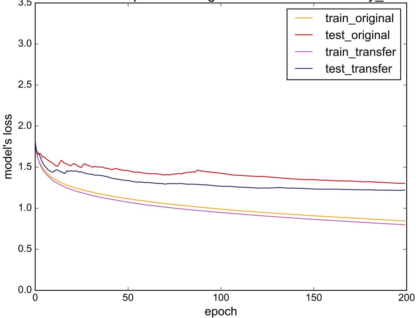
Source: Computers - Target: uWaveGestureLibrary_Y
