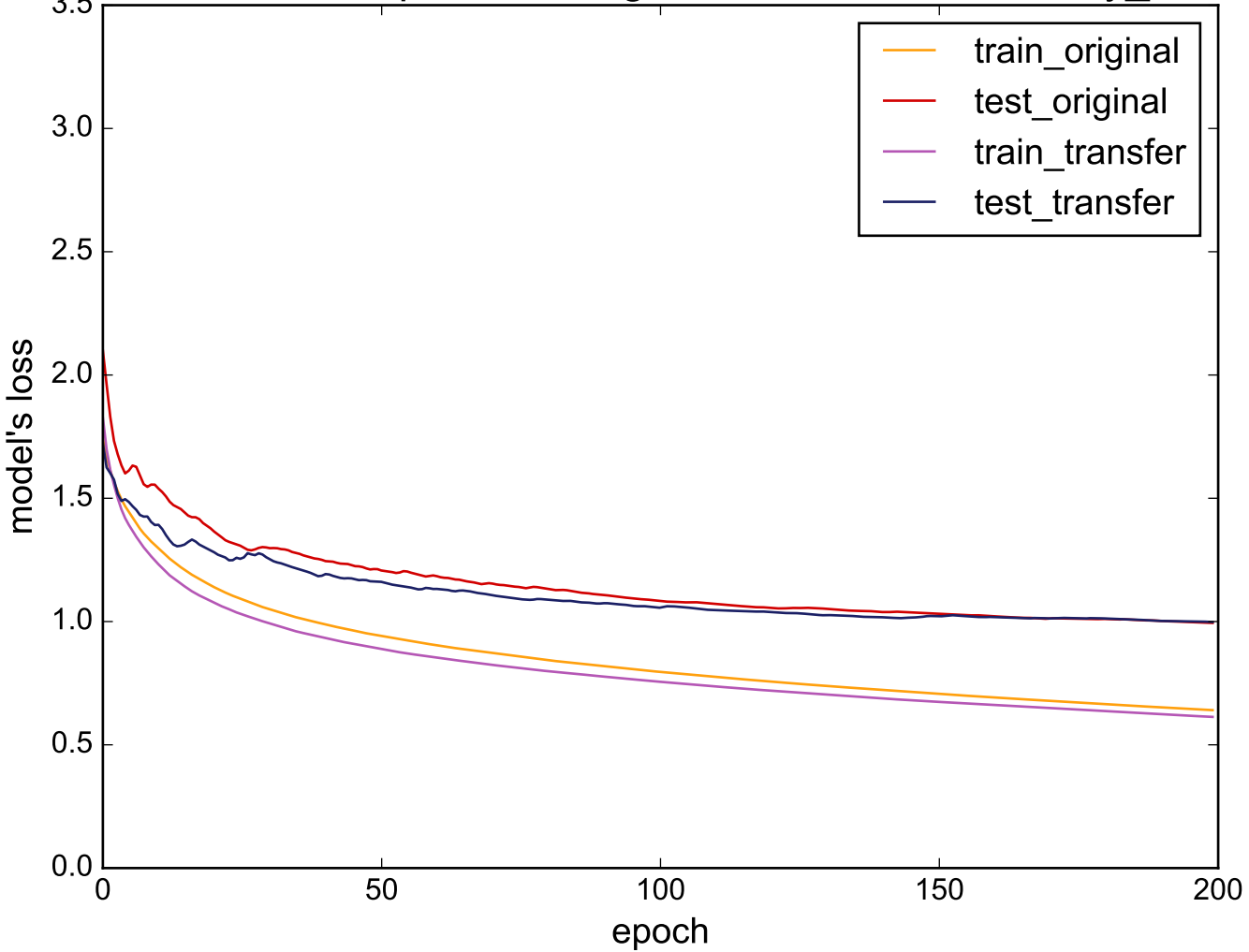
Source: Computers - Target: uWaveGestureLibrary_Z
