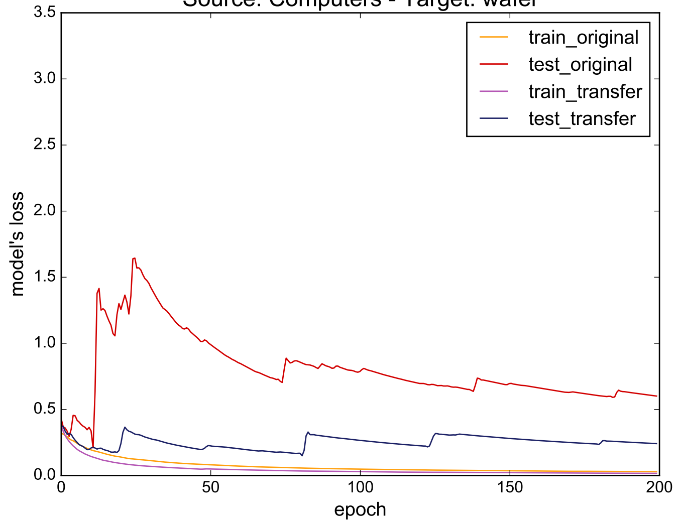
Source: Computers - Target: wafer
