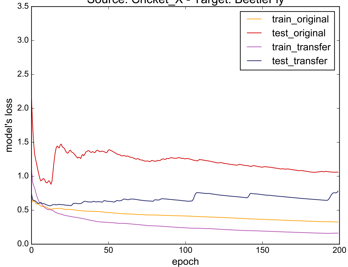
Source: Cricket_X - Target: BeetleFly
