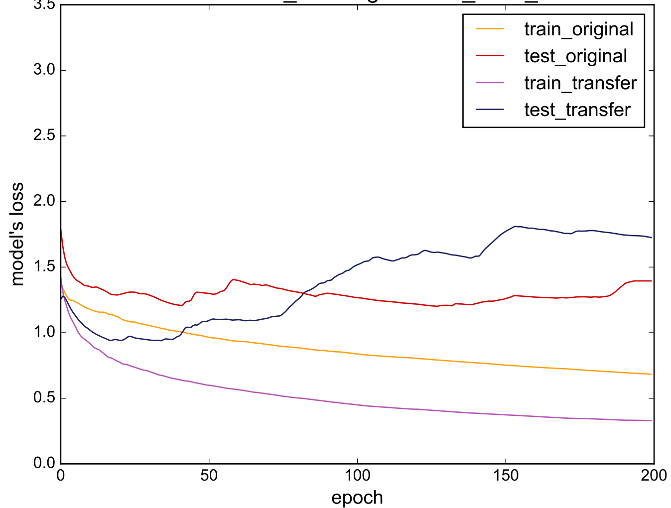
Source: Cricket_X - Target: CinC_ECG_torso
