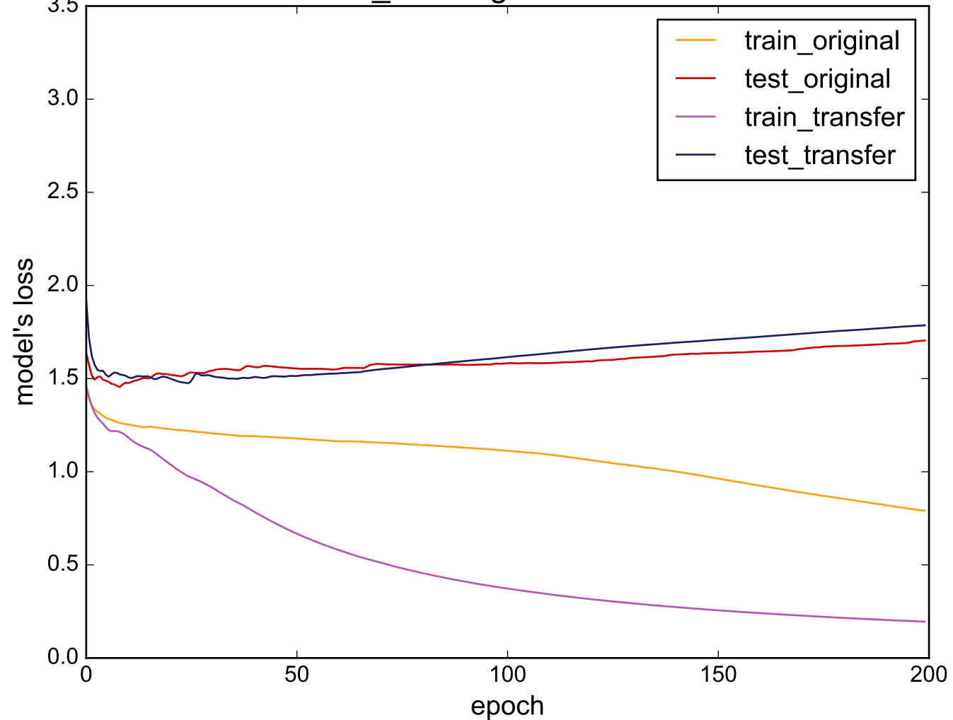
Source: Cricket_X - Target: DiatomSizeReduction
