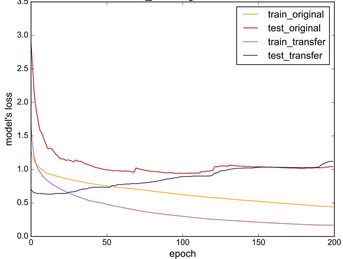
Source: Cricket_X - Target: DistalPhalanxTW
