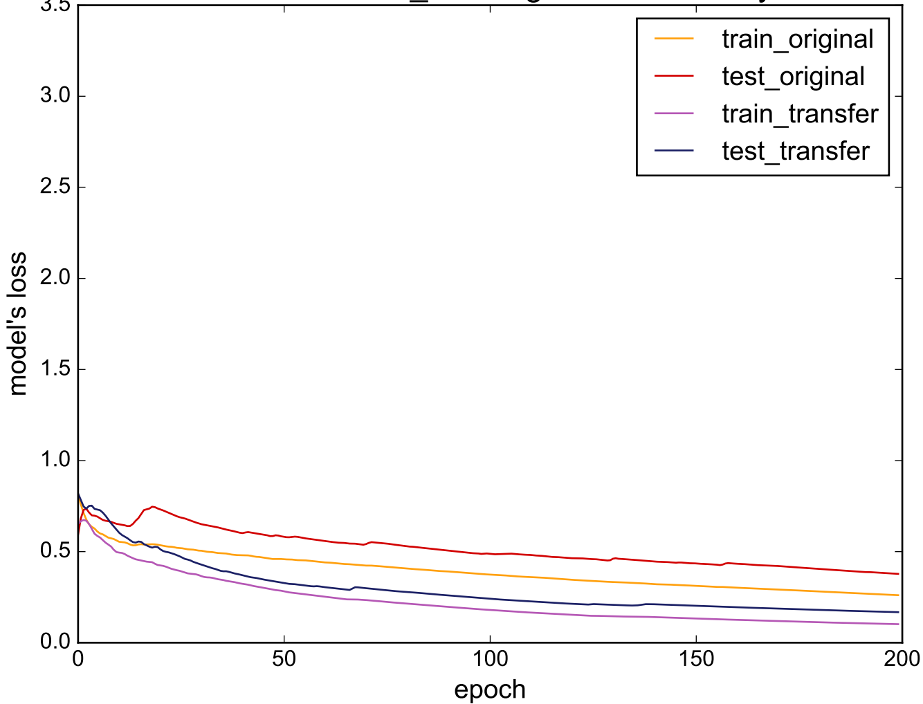
Source: Cricket_X - Target: ECGFiveDays
