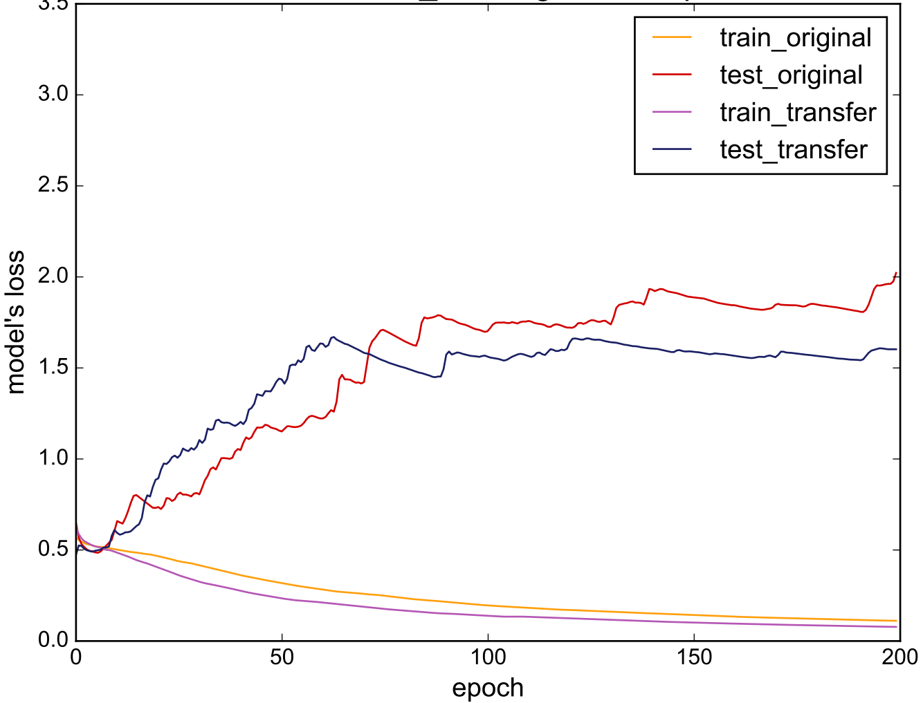
Source: Cricket_X - Target: Earthquakes
