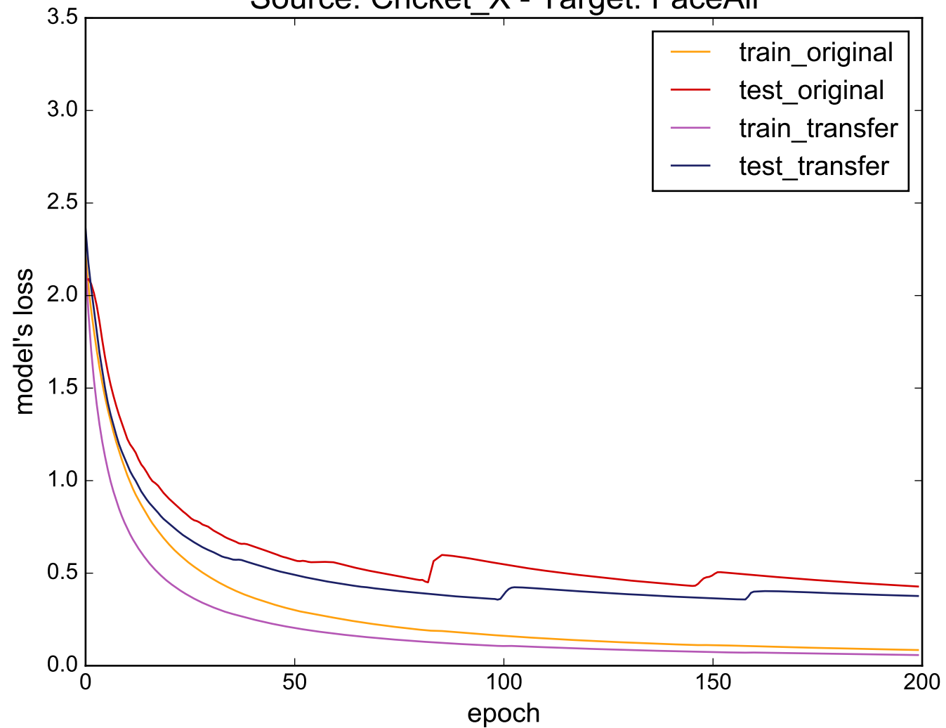
Source: Cricket_X - Target: FaceAll
