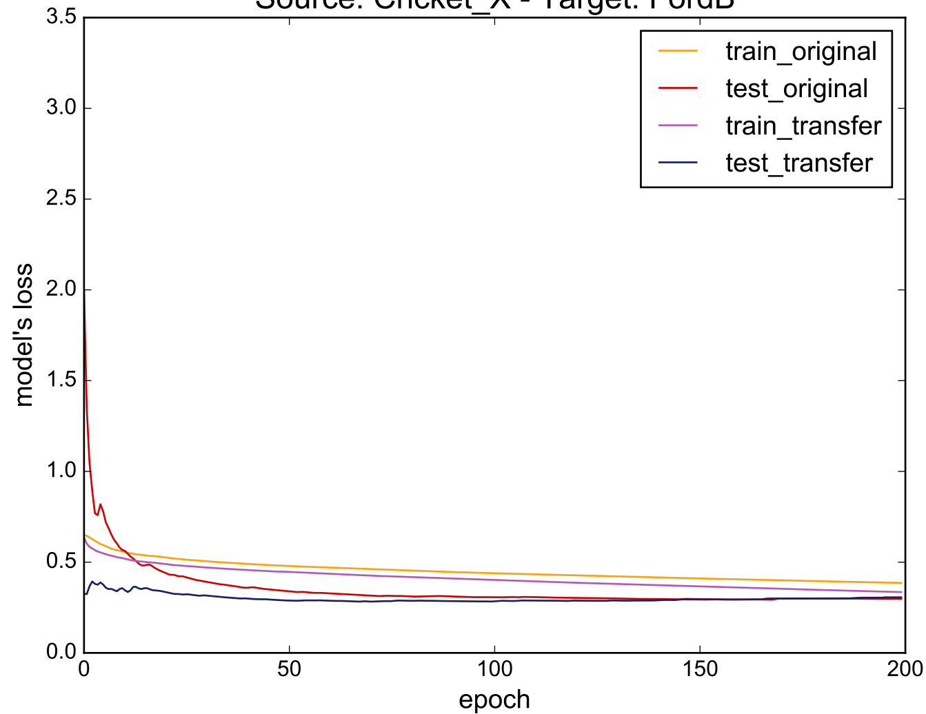
Source: Cricket_X - Target: FordB
