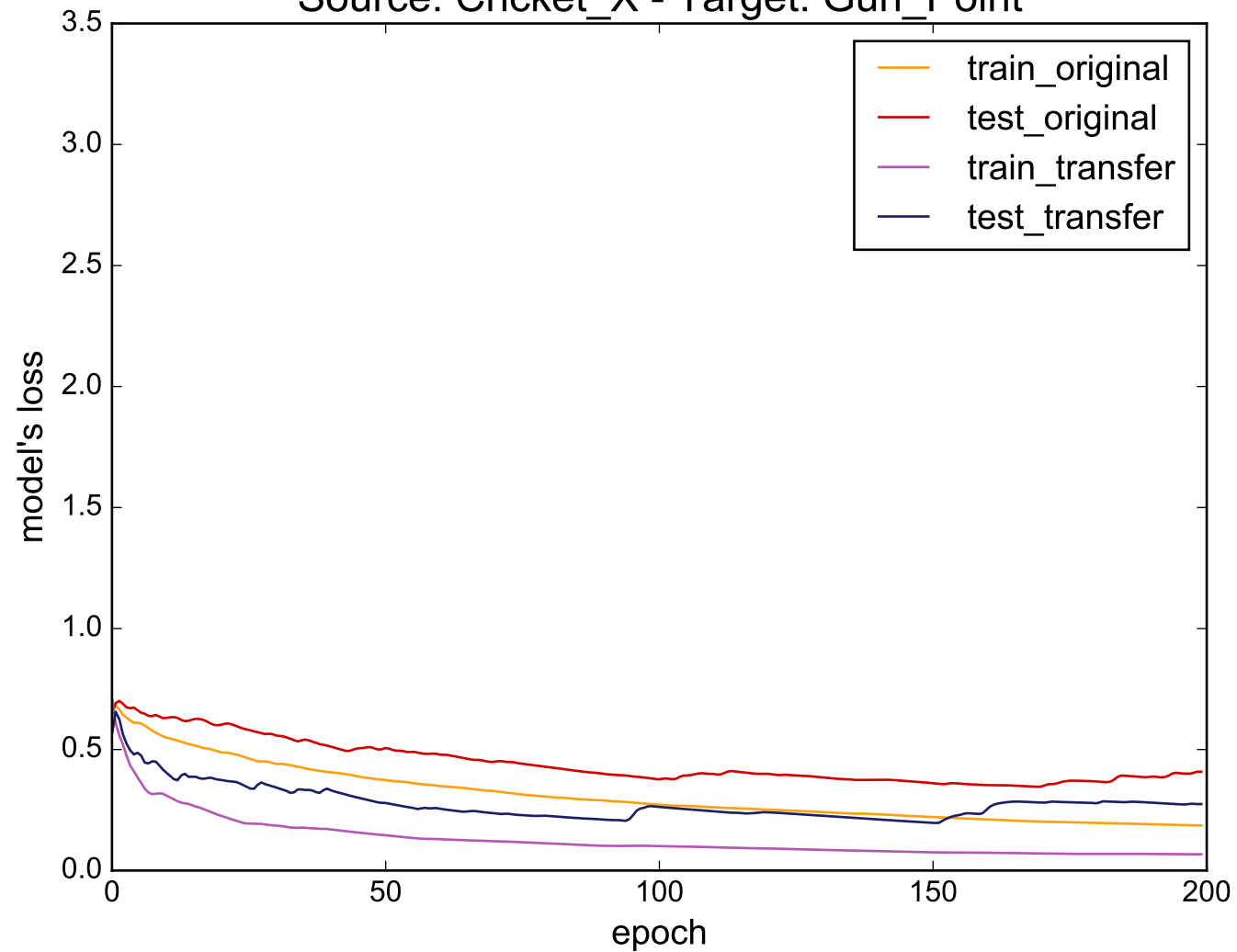
Source: Cricket_X - Target: Gun_Point
