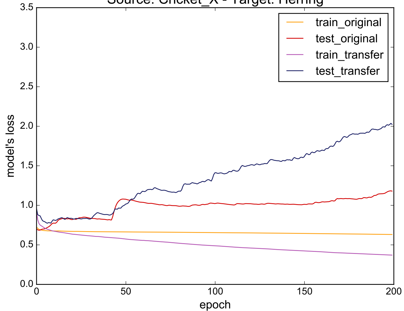
Source: Cricket_X - Target: Herring
