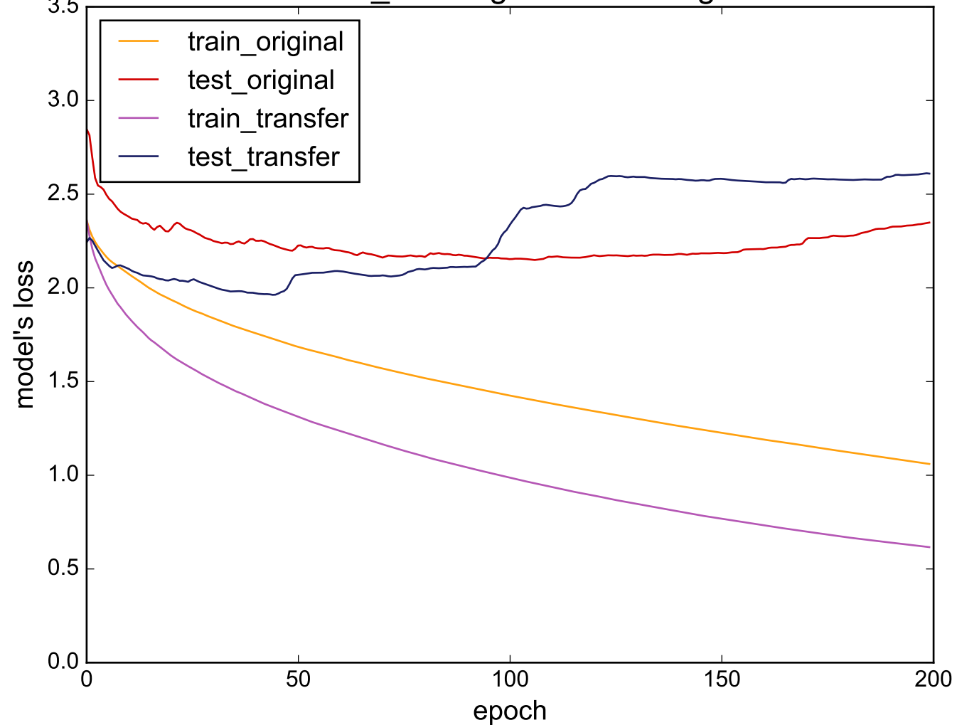
Source: Cricket_X - Target: InsectWingbeatSound
