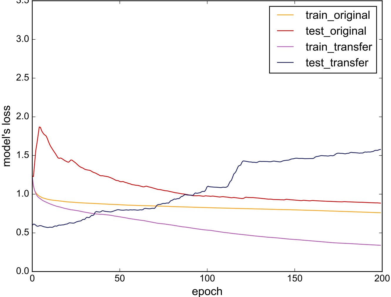
Source: Cricket_X - Target: MiddlePhalanxOutlineAgeGroup
