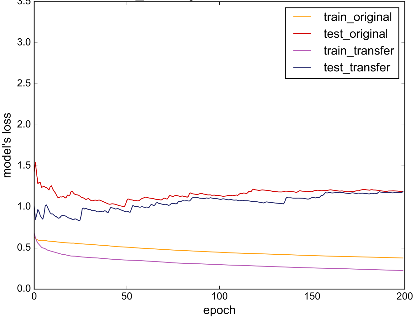
Source: Cricket_X - Target: MiddlePhalanxOutlineCorrect
