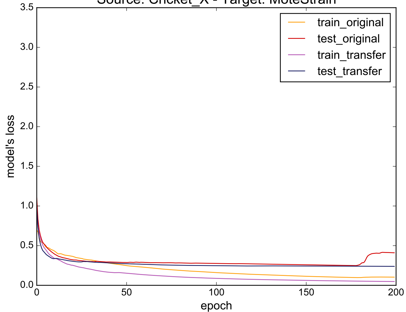
Source: Cricket_X - Target: MoteStrain
