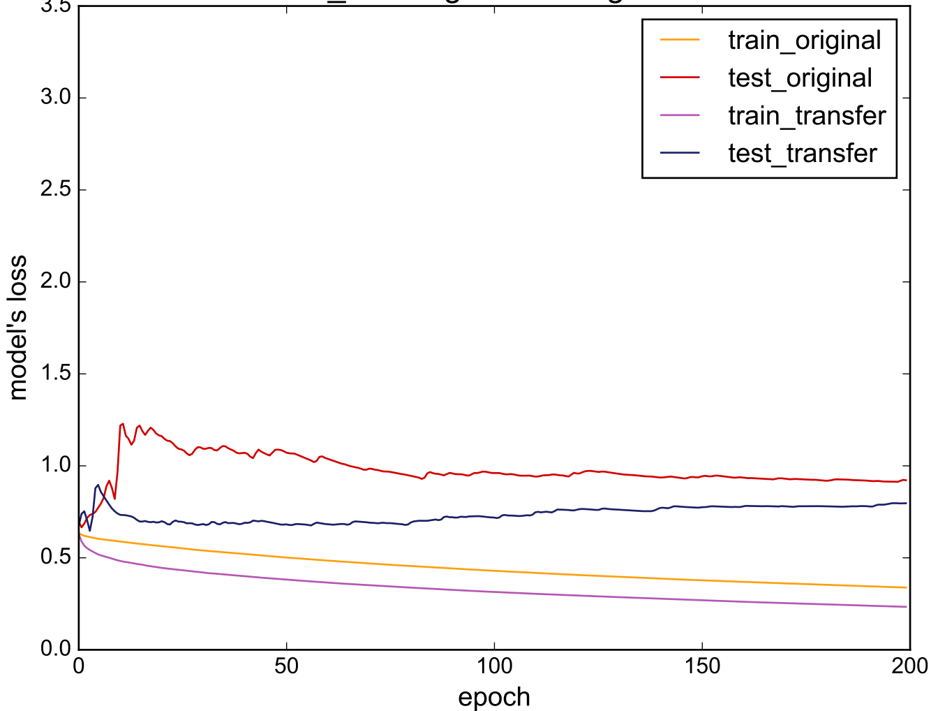
Source: Cricket_X - Target: PhalangesOutlinesCorrect
