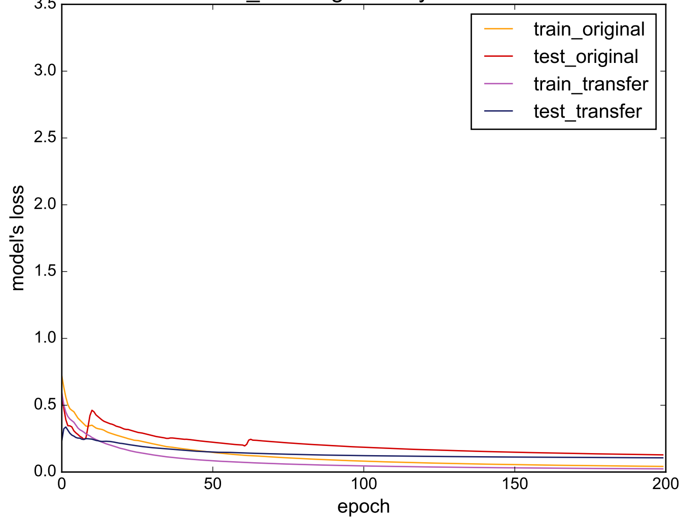
Source: Cricket_X - Target: SonyAIBORobotSurfacell
