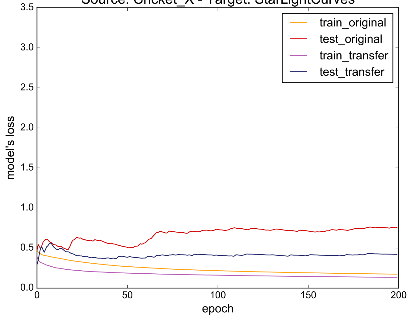
Source: Cricket_X - Target: StarLightCurves
