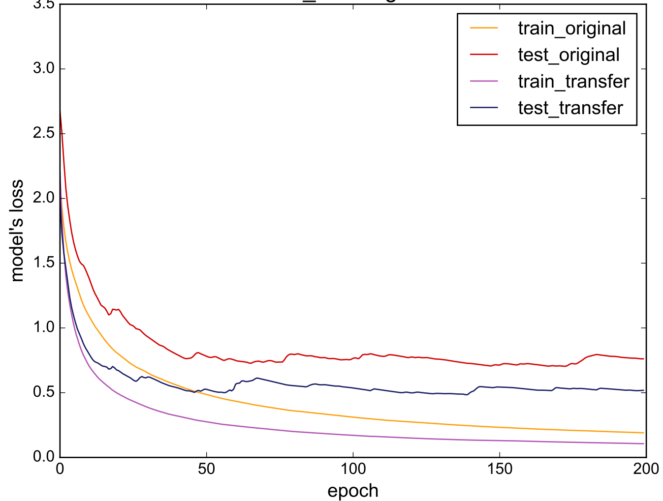
Source: Cricket_X - Target: SwedishLeaf
