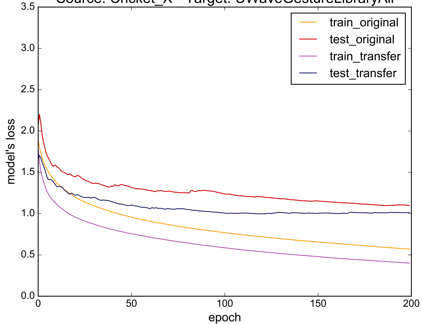
Source: Cricket_X - Target: UWaveGestureLibraryAll
