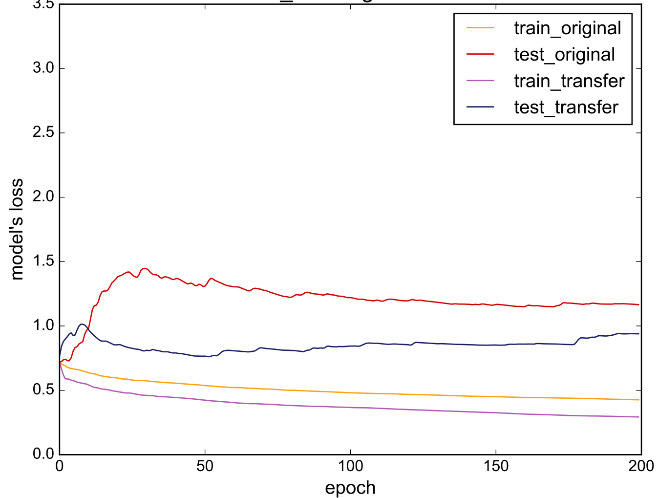
Source: Cricket_X - Target: WormsTwoClass
