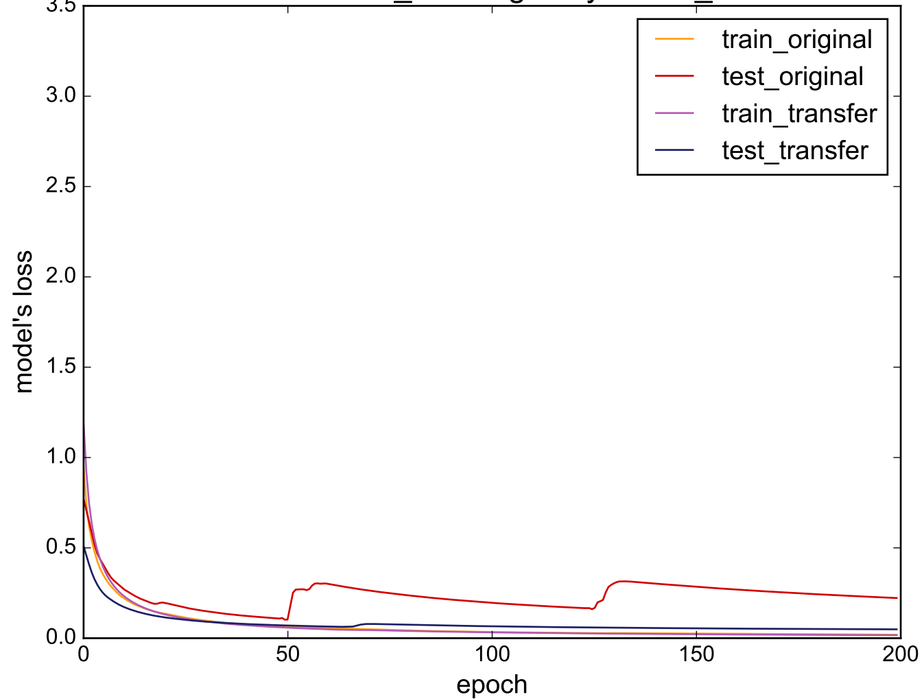
Source: Cricket_X - Target: synthetic_control
