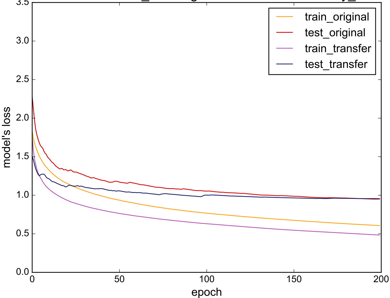
Source: Cricket_X - Target: uWaveGestureLibrary_X
