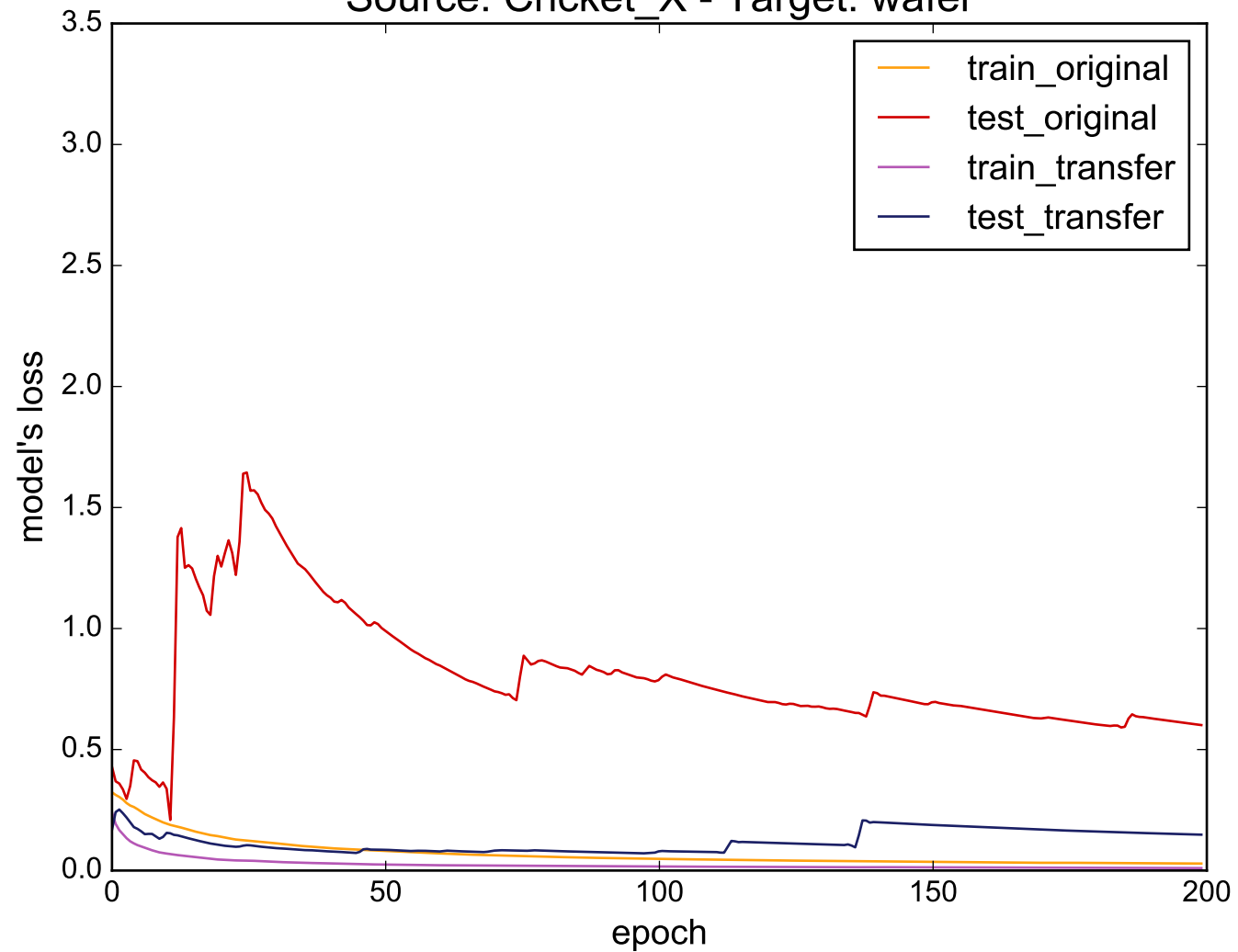
Source: Cricket_X - Target: wafer
