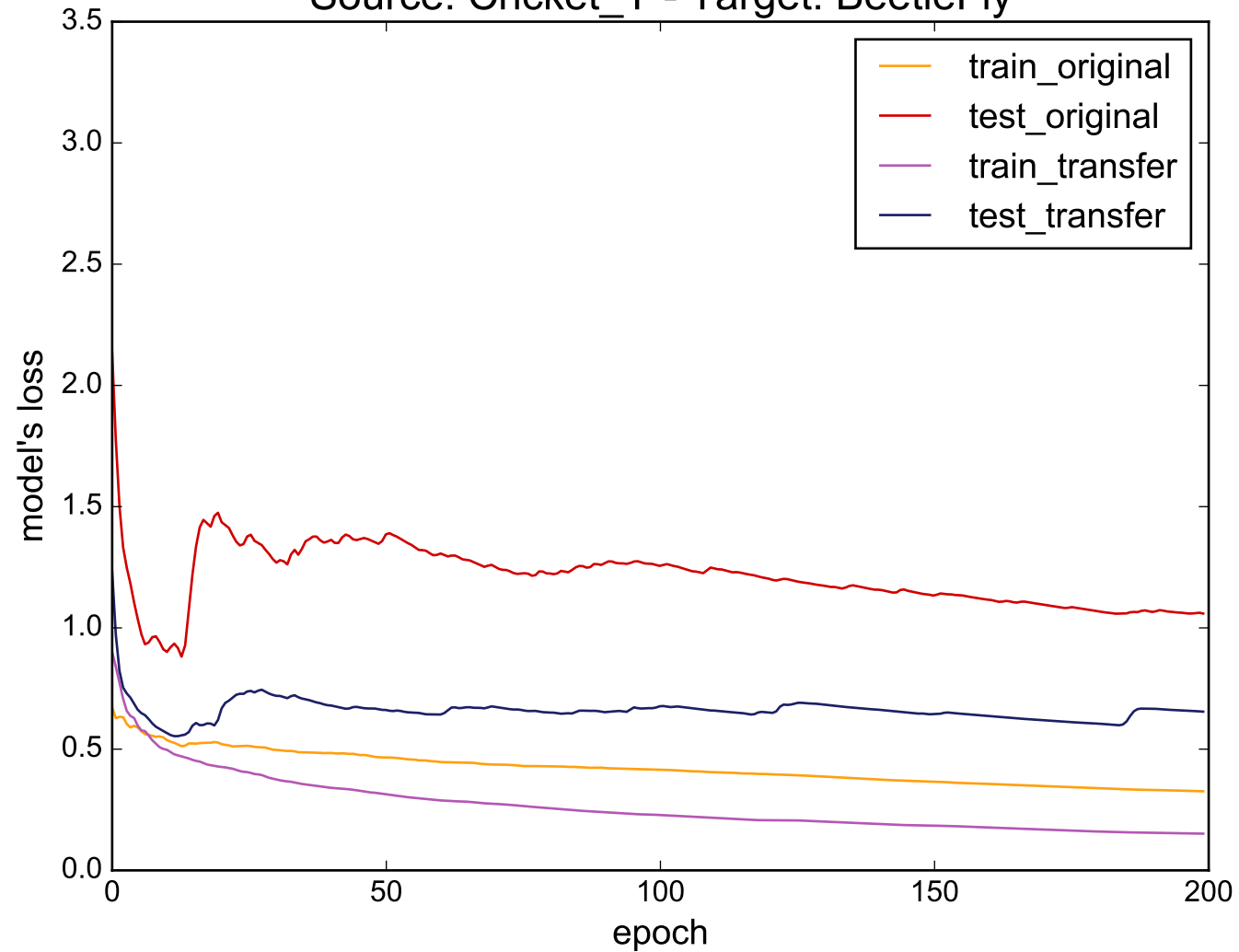
Source: Cricket_Y - Target: BeetleFly
