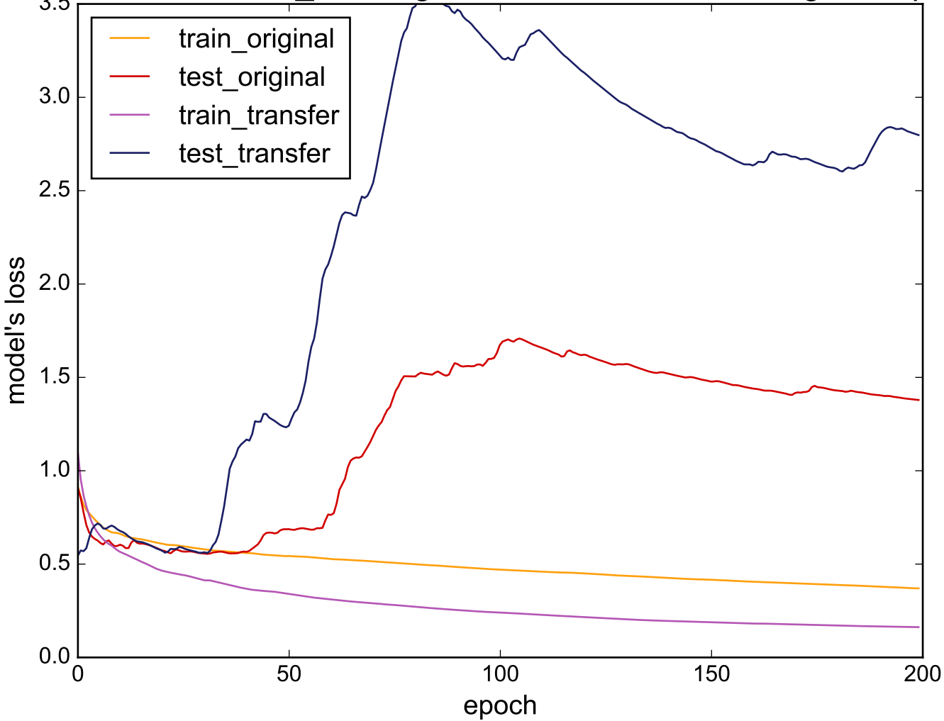
Source: Cricket_Y - Target: DistalPhalanxOutlineAgeGroup
