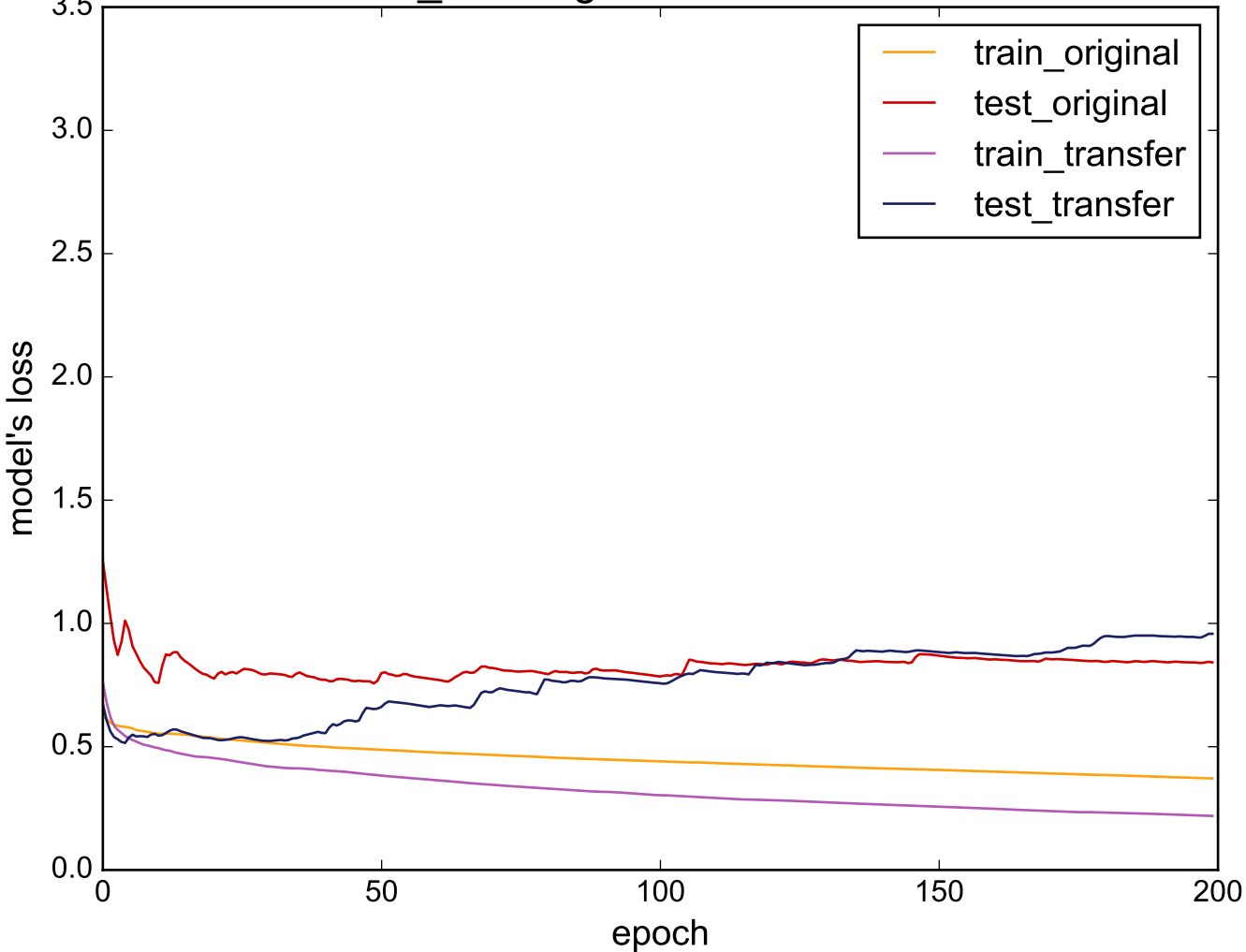
Source: Cricket_Y - Target: DistalPhalanxOutlineCorrect
