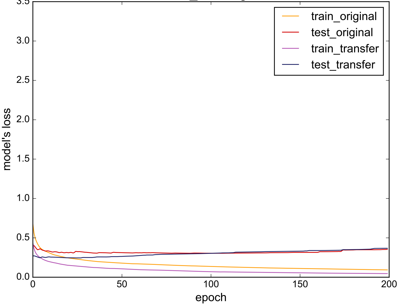
Source: Cricket_Y - Target: ECG5000
