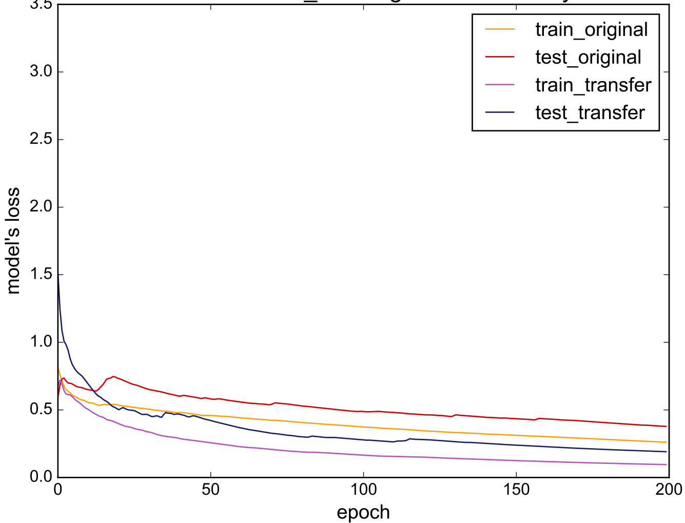
Source: Cricket_Y - Target: ECGFiveDays
