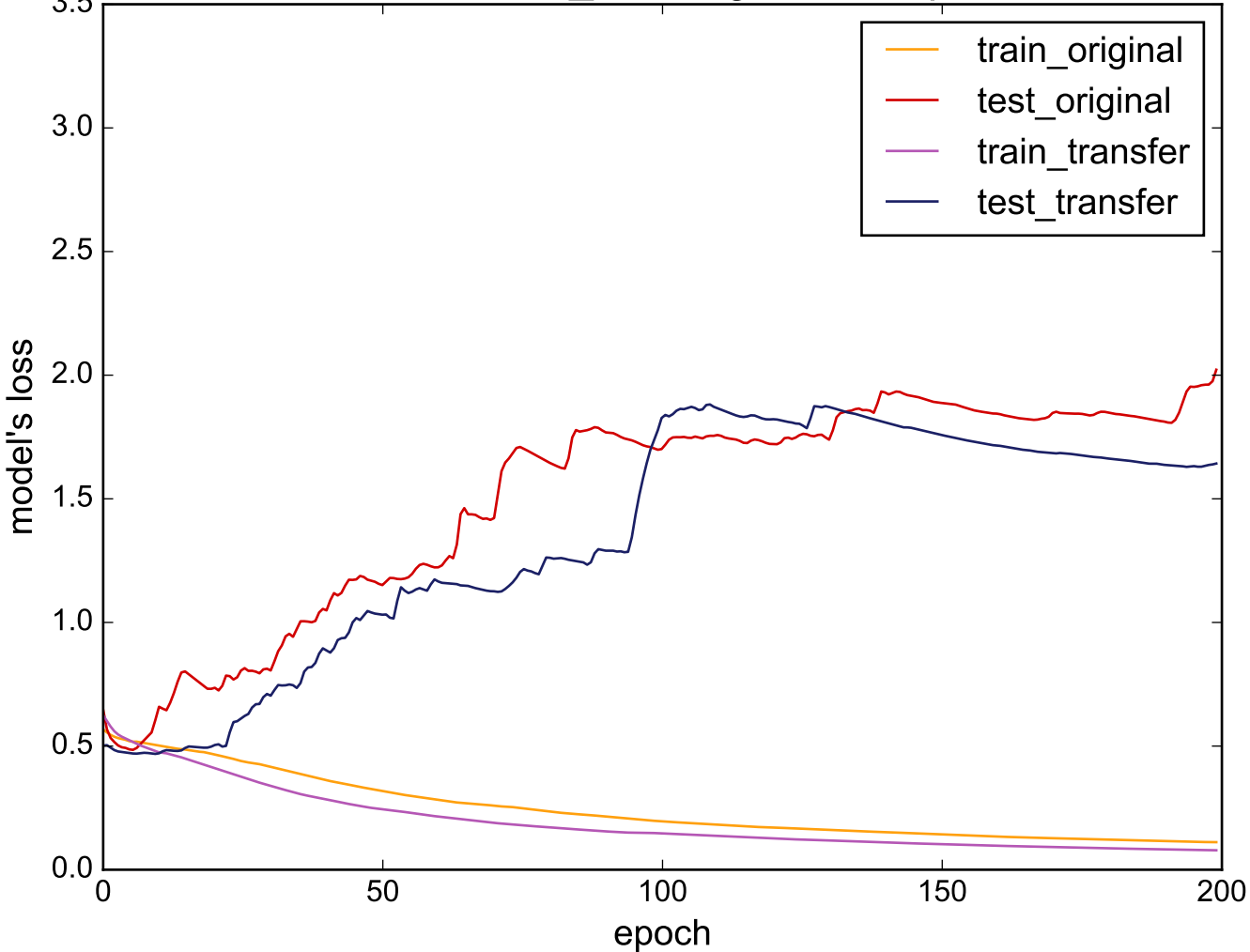
Source: Cricket_Y - Target: Earthquakes
