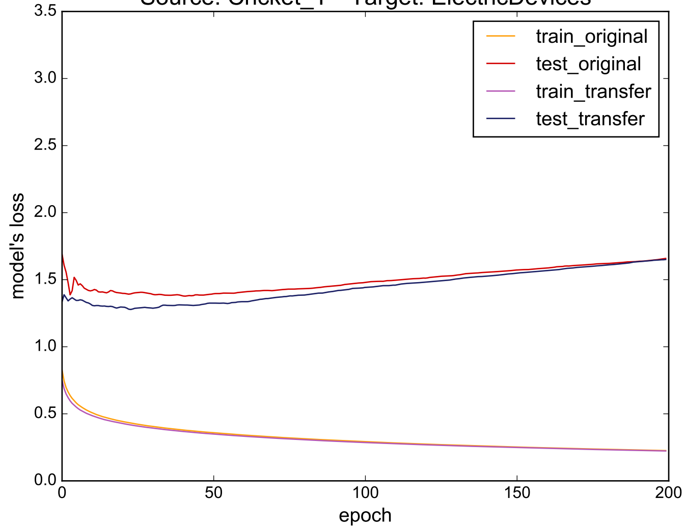
Source: Cricket_Y - Target: ElectricDevices
