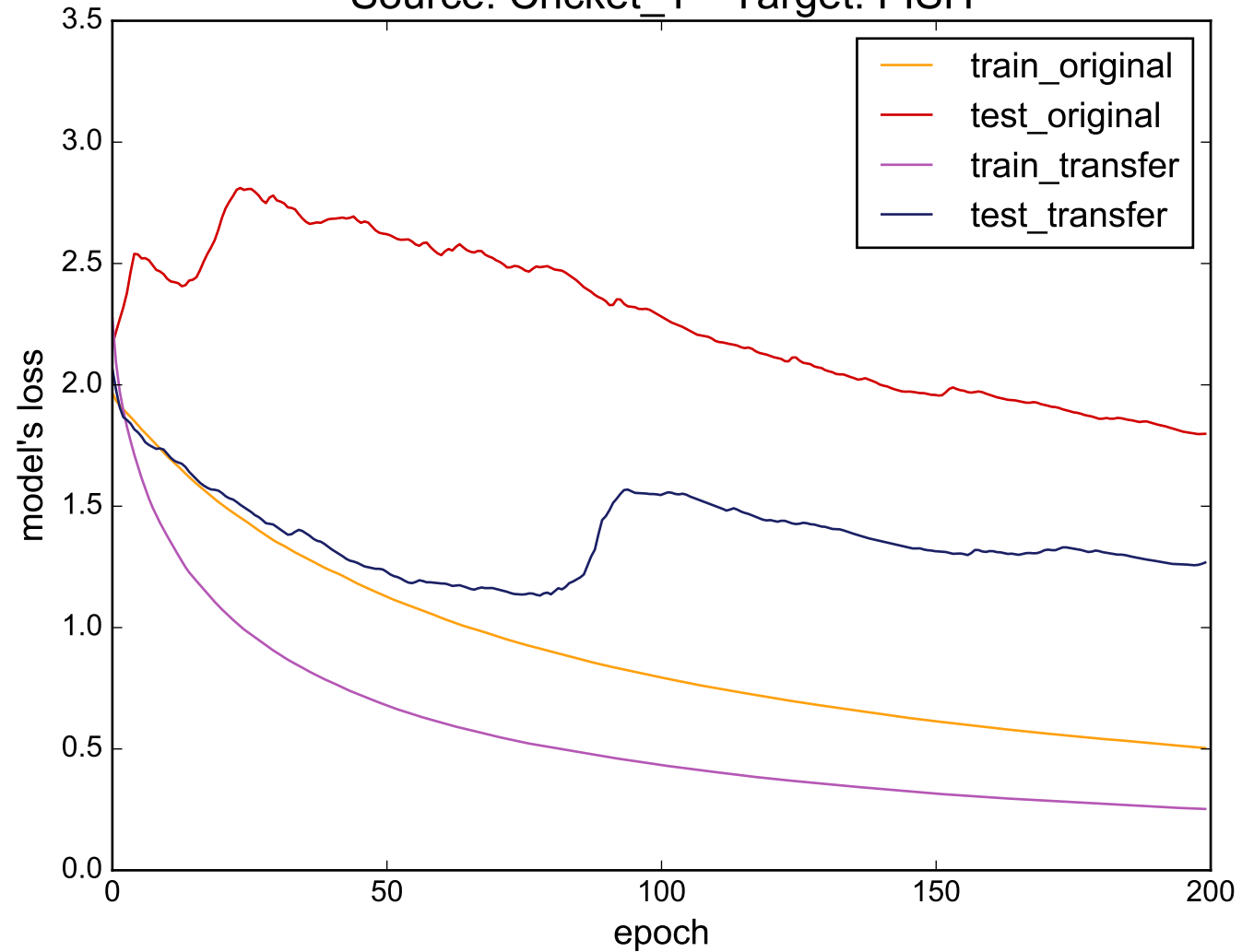
Source: Cricket_Y - Target: FISH
