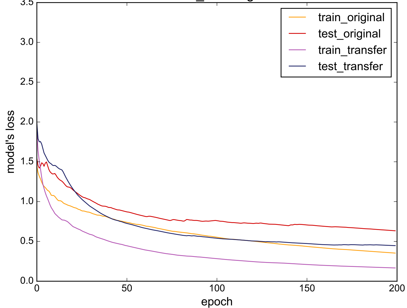
Source: Cricket_Y - Target: FaceFour
