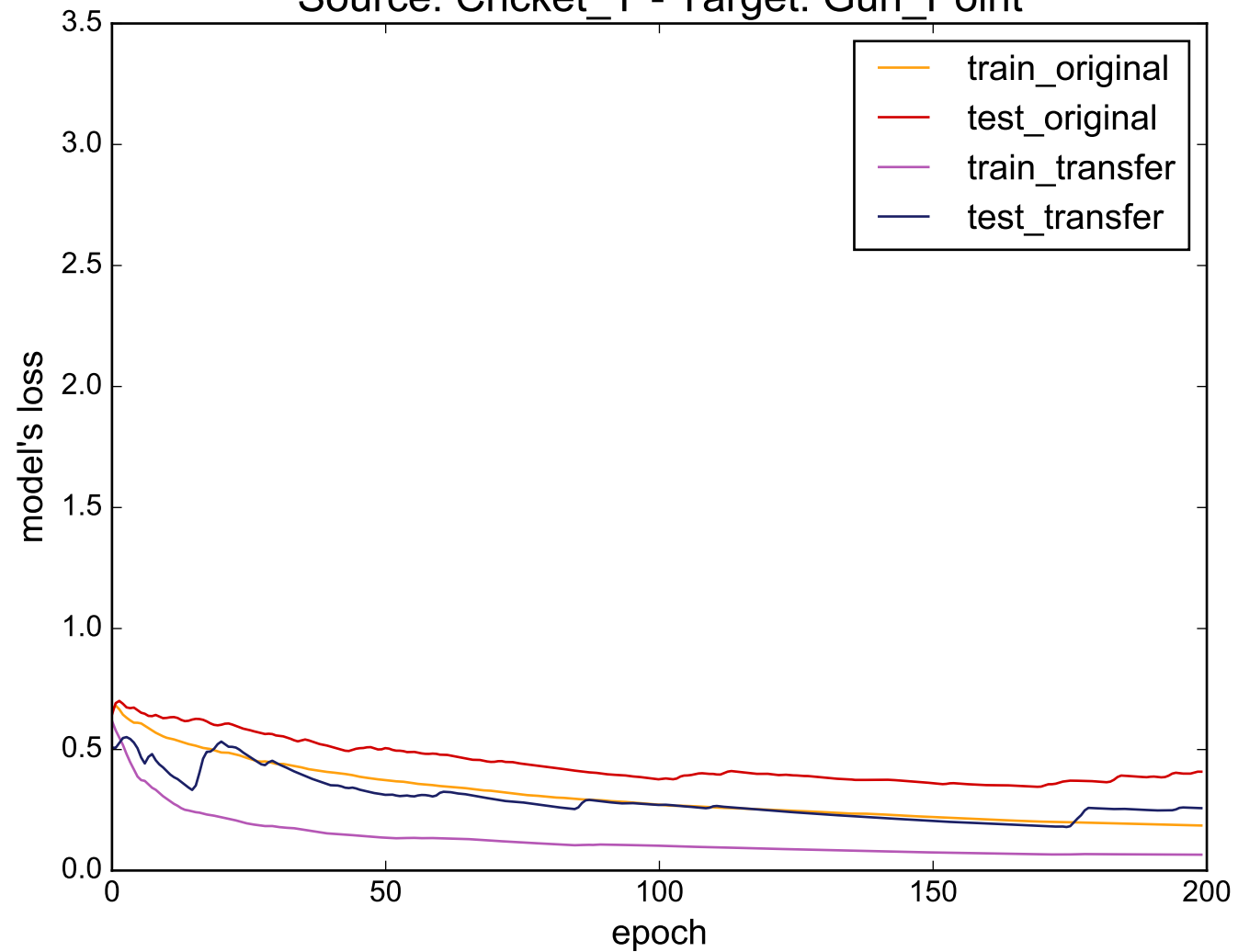
Source: Cricket_Y - Target: Gun_Point
