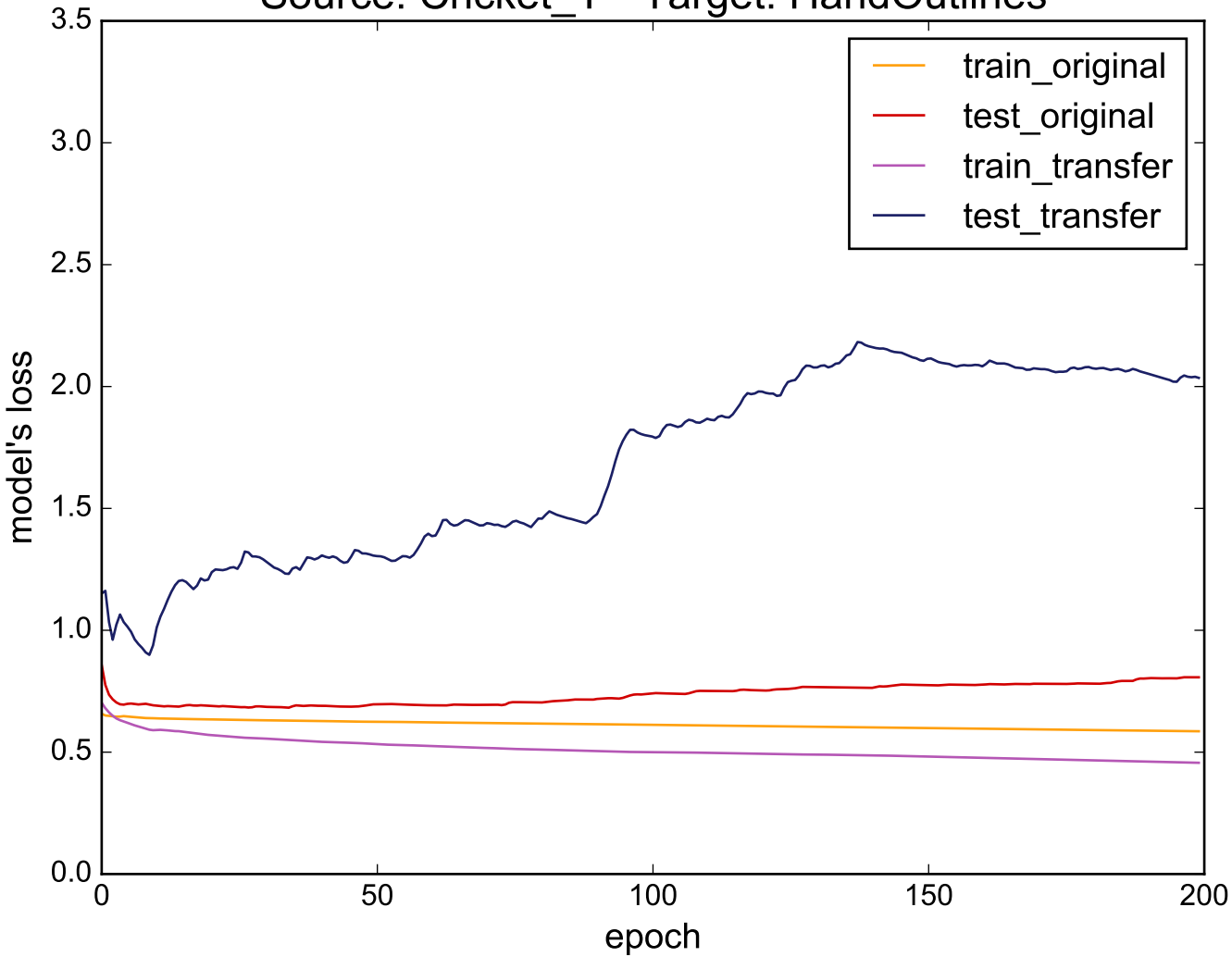
Source: Cricket_Y - Target: HandOutlines
