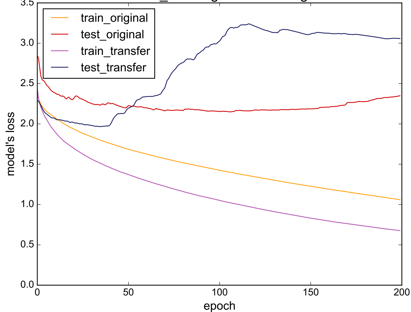
Source: Cricket_Y - Target: InsectWingbeatSound
