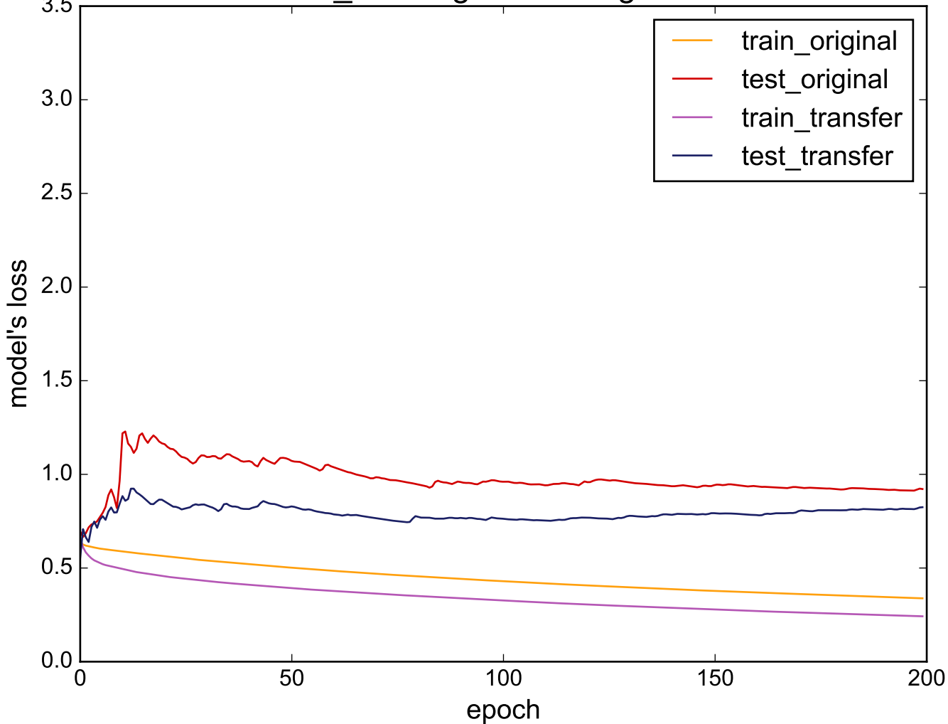
Source: Cricket_Y - Target: PhalangesOutlinesCorrect
