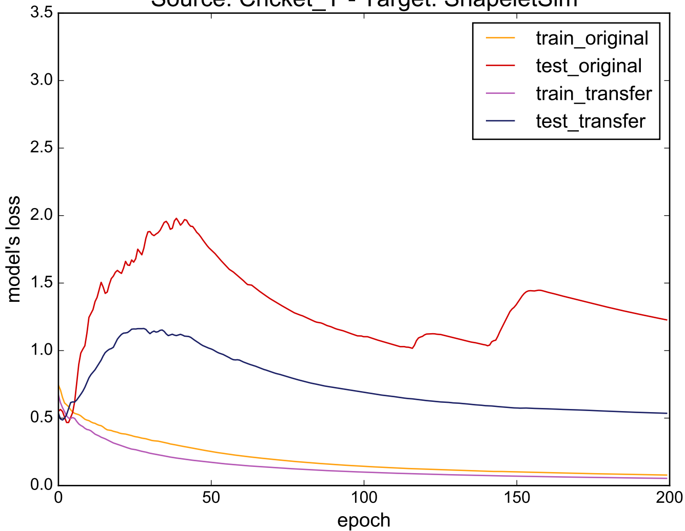
Source: Cricket_Y - Target: ShapeletSim
