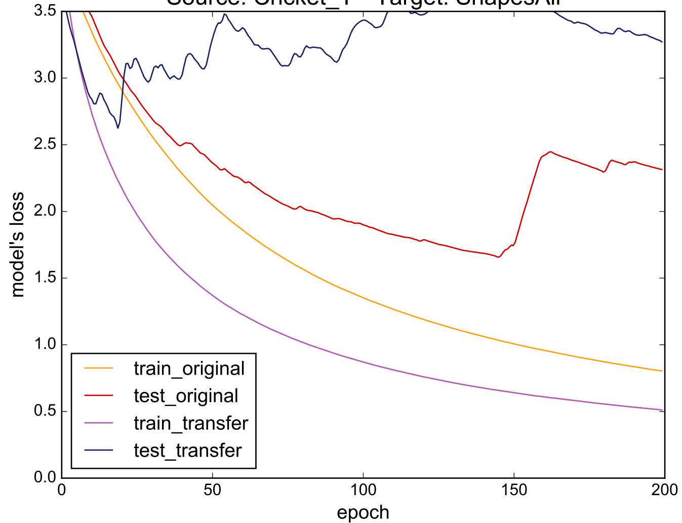
Source: Cricket_Y - Target: ShapesAll
