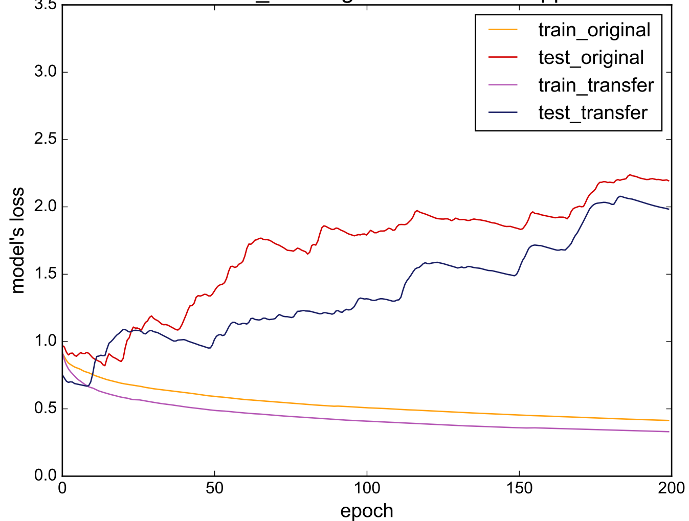
Source: Cricket_Y - Target: SmallKitchenAppliances
