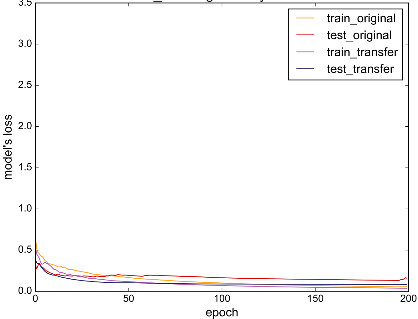
Source: Cricket_Y - Target: SonyAIBORobotSurface
