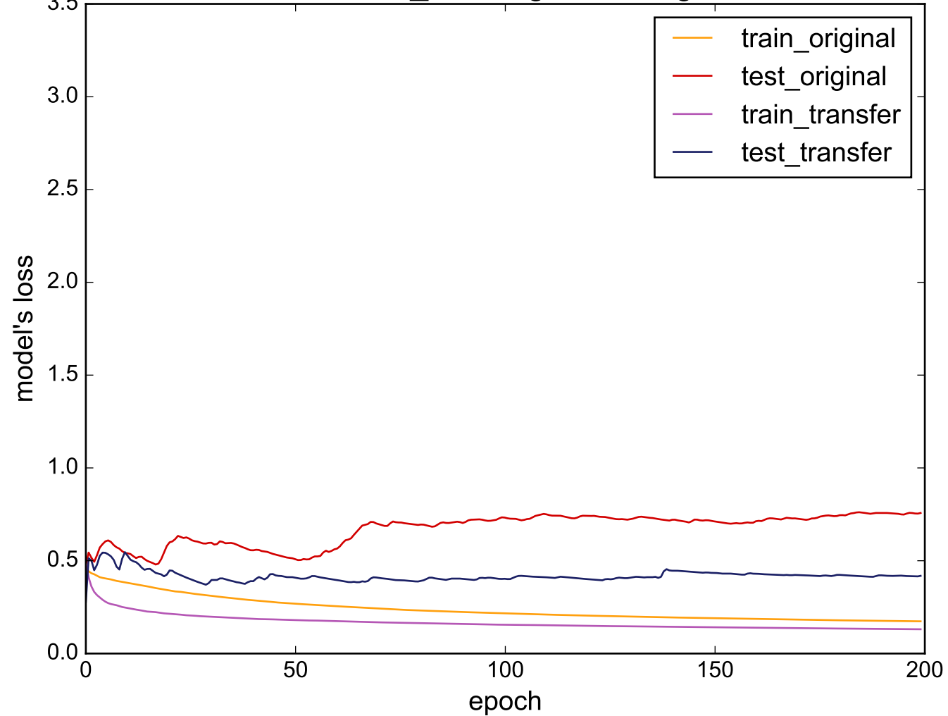
Source: Cricket_Y - Target: StarLightCurves
