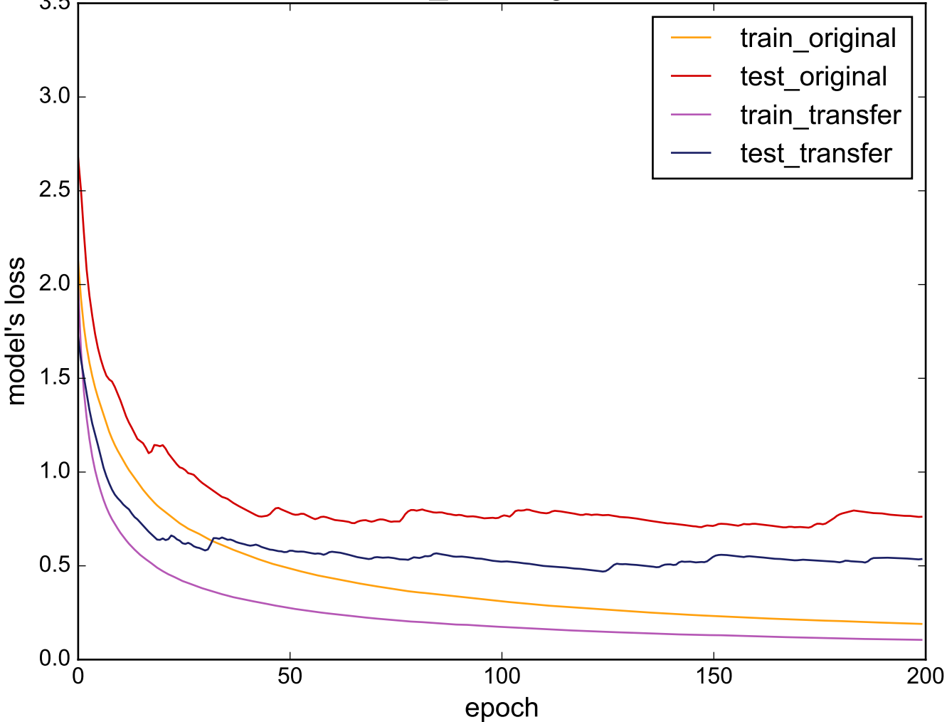
Source: Cricket_Y - Target: SwedishLeaf
