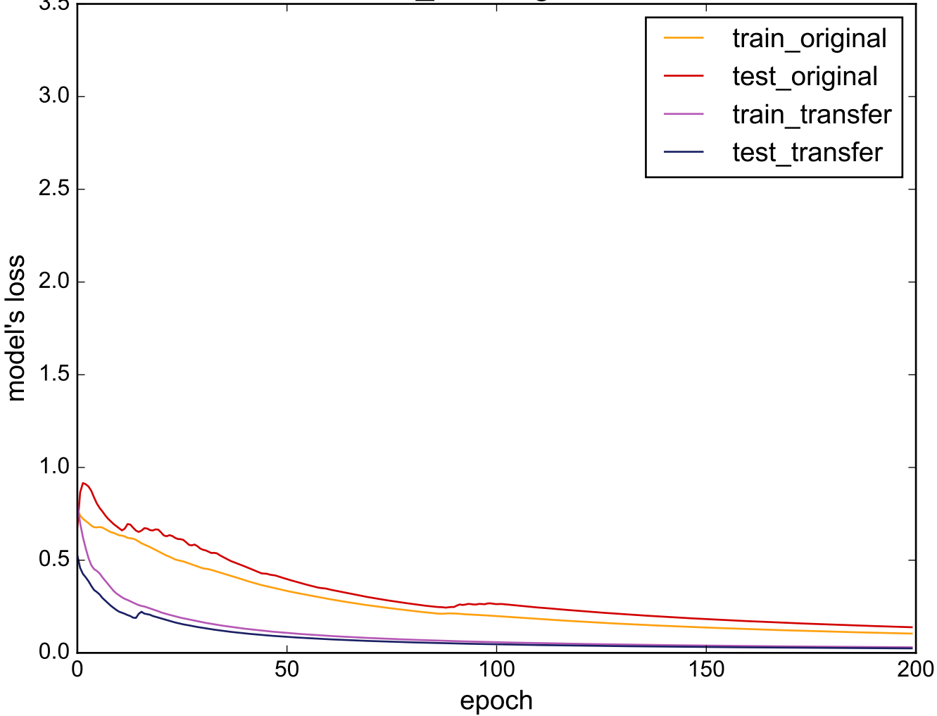
Source: Cricket_Y - Target: TwoLeadECG
