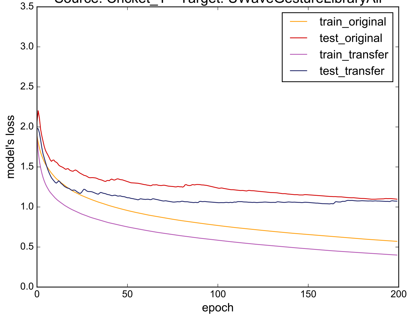
Source: Cricket_Y - Target: UWaveGestureLibraryAll
