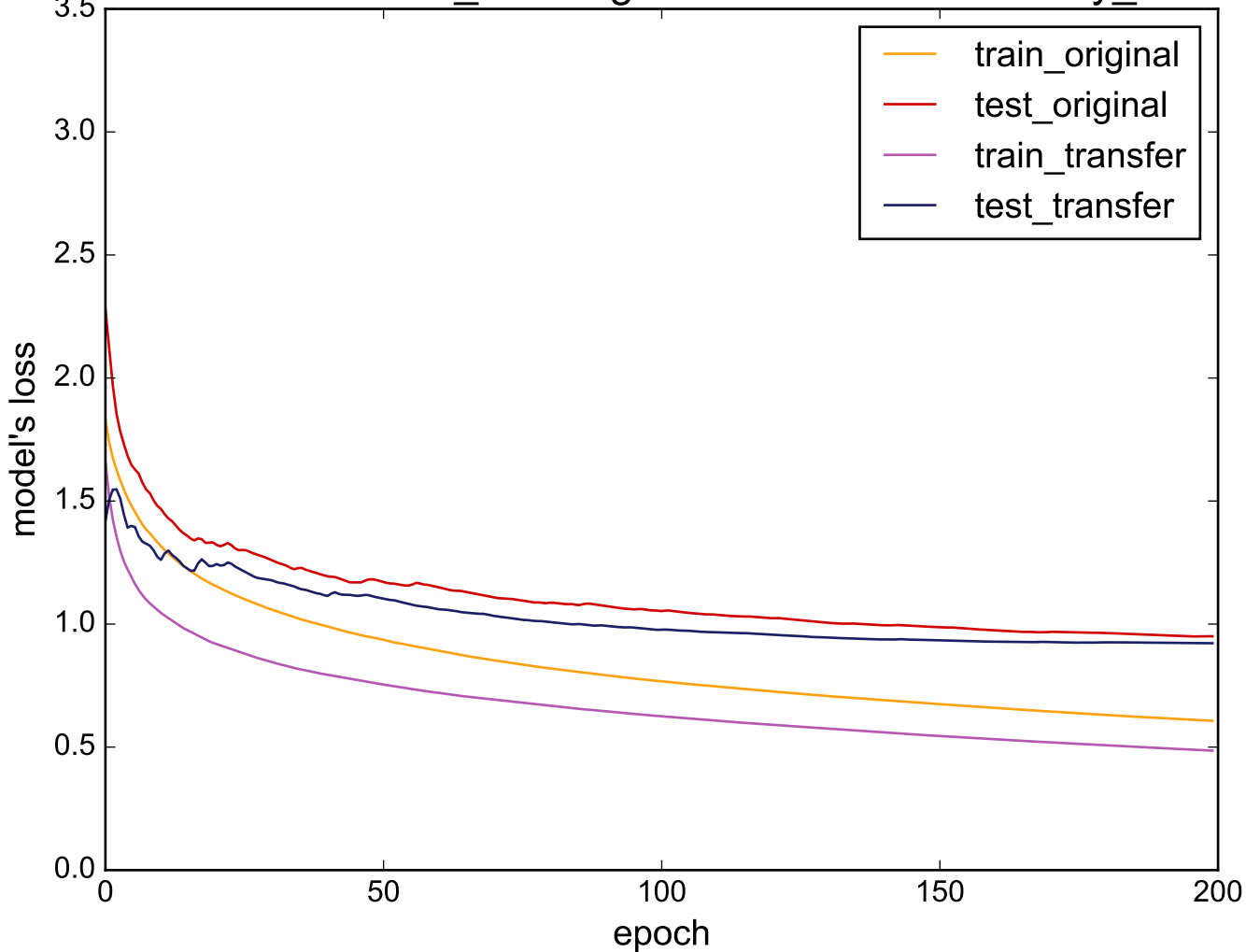
Source: Cricket_Y - Target: uWaveGestureLibrary_X
